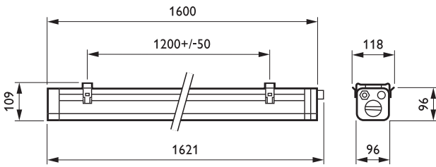
WT360C 2xTL5-49W/840 HFP C
