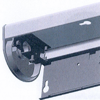
Use hooks for assembly plate while installing cables
