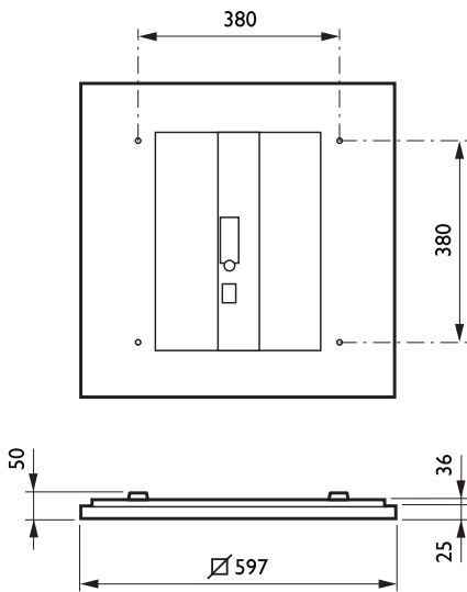
SM120V LED34S/830 PSD W60L60 VAR-PC
