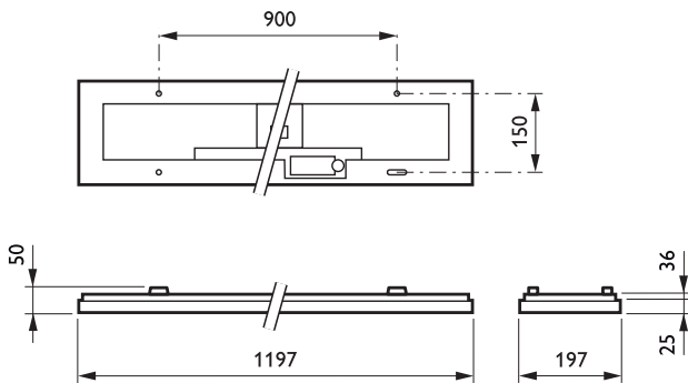
SM120V LED37S/840 PSD W20L120
