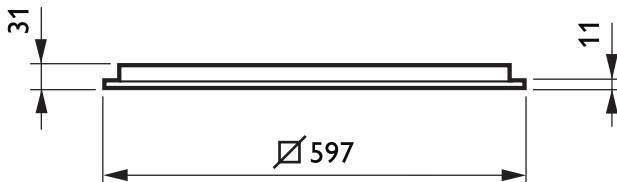
RC120B LED26S/840 PSD W60L60
