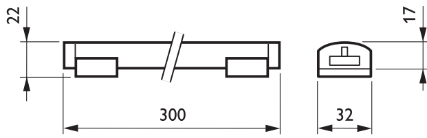
SM440L I 10xLED-HB/4000K 24V CE, UL
