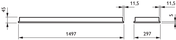
TBS460 2x35W/840 HFP C8 PI IP
