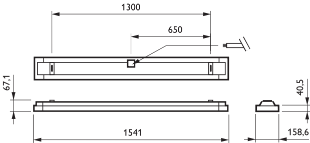
TCS260 1x49W/830 HFS M2 WH
