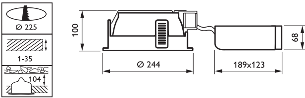
FBS291 2xPL-C/4P18W/840 HFP FR PI WH
