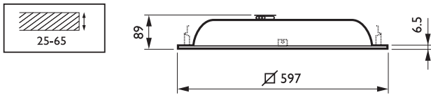
TBS741 1xTL5C60W/830 HFP P IP VH
