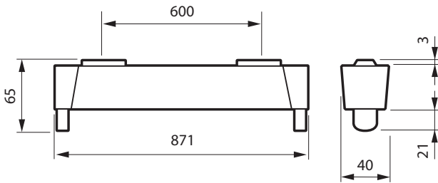
TMS122 1xTL5-39W/830 HFP
