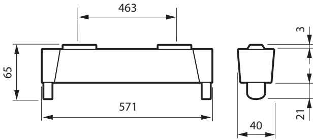
TMS122 1xTL5-14W/840 HFP TW1
