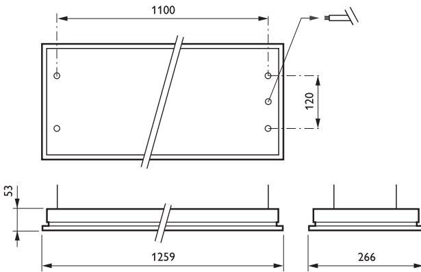
TPS772 3x54W/827/865 HFD AC-MLO SMS
