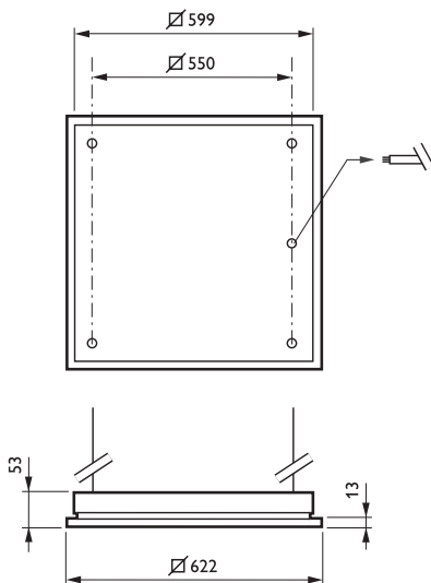
TPS760 4x14W/830 HFR ND AC-MLO SM4
