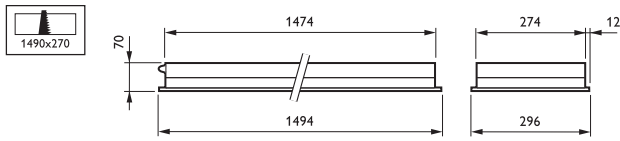
TBS424 2xTL5-49W/830 HFP C5-H GT IP65
