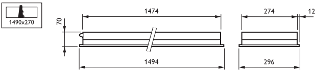
TBS424 2xTL5-35W/830 HFP C5-H GT IP65
