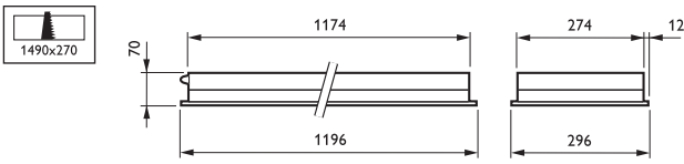
TBS424 2xTL5-28W/830 HFP C5-H GT IP65
