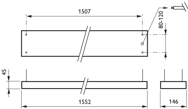
TPS642 1x49W/830 HFP D8-VH SMS ALU
