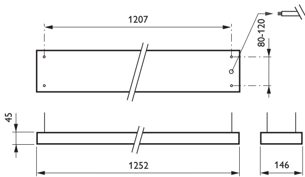
TPS640 1x54W/830 HFR AC-MLO SM2 ALU
