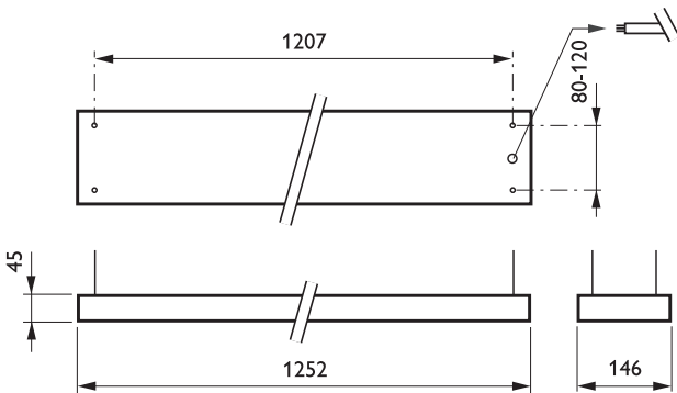
TPS640 1x54W/830 HFP M2 SM2 ALU
