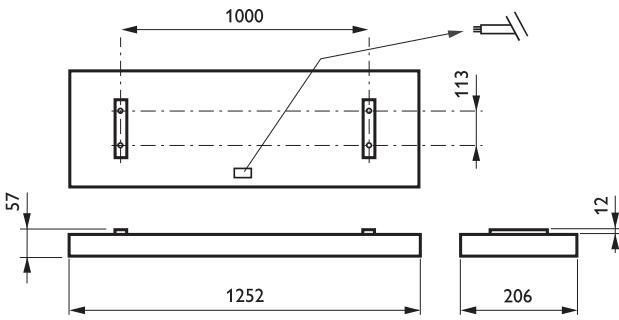
TCS640 2x54W/830 HFP M2 ALU
