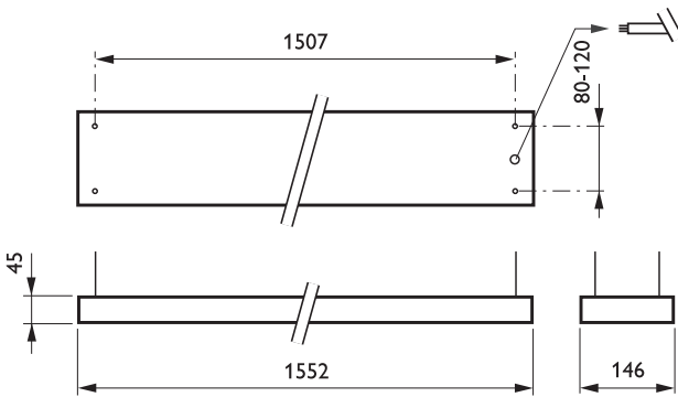
TPS640 1x35W/830 HFP D8 SMS ALU
