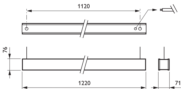
TPS682 1x28VV/830 HFR AC-MLO SM2 ALU
