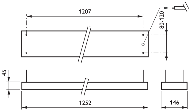
TPS642 1x54W/830 HFP D8 SM2 ALU
