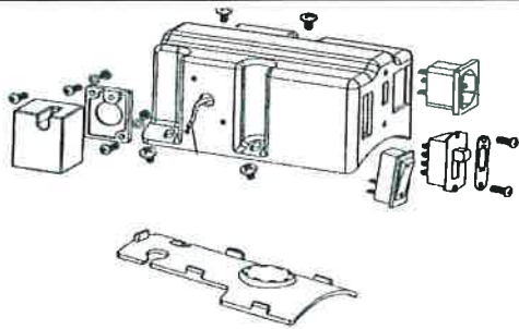
Box capacitor + switches PMK-36-ALL
