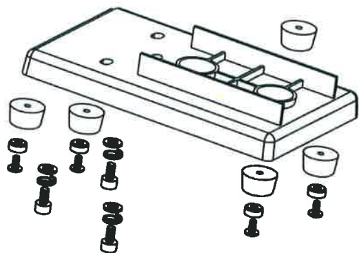
Complete base plate PMK-23-700 for MK-40-60 PMK-23-890 for MK-120-180-240-280
