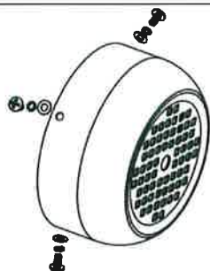
Steel protection fan & screws PMK-24-700 for MK-40-60 PMK-24-120 for MK-120 PMK-24-900 for MK-180-240-280
