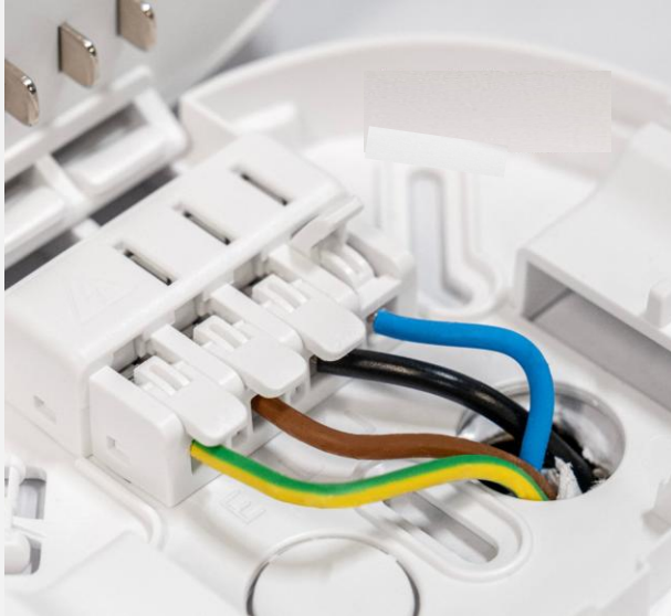
PUSH-IN WIRE
