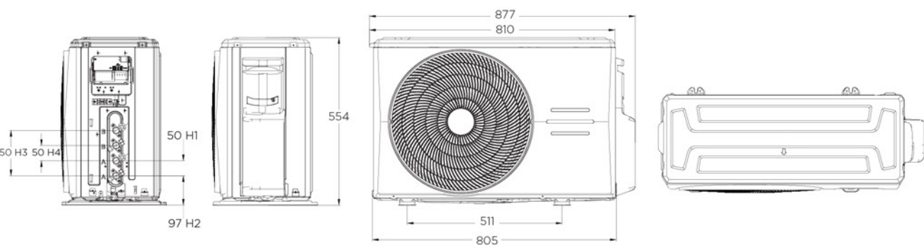
M2OF-18HFN8-Q Dimensional Drawings
