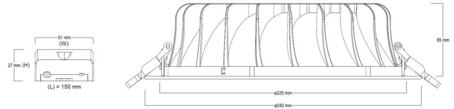
Syl-Lighter LED II 240
