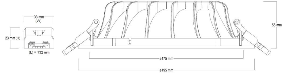
Syl-Lighter LED II 195
