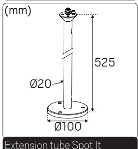
Extension tube Spot It
