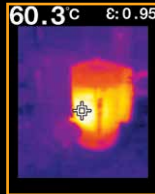
Mechanical Overheating
