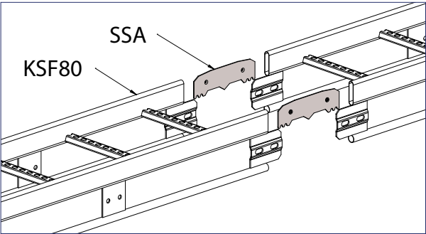
Joint SSA is a reinforcing piece for cable ladder KS80 and KSF80 joints.
