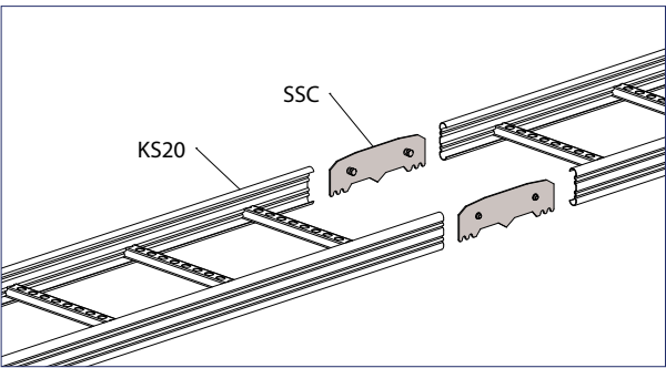
KS20 cable ladders can be attached together with joint SSC.
