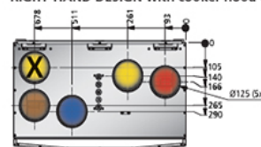
RIGHT-HAND DESIGN with cooker hood connection
