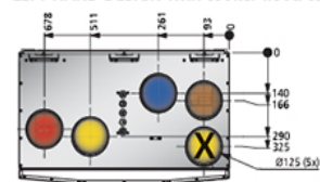
LEFT-HAND DESIGN with cooker hood connection
