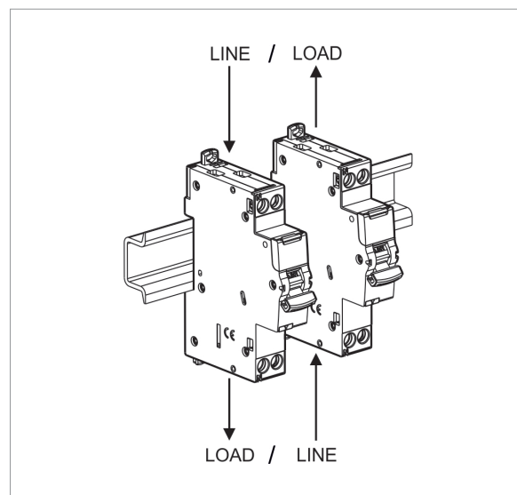
Connection Diagram
