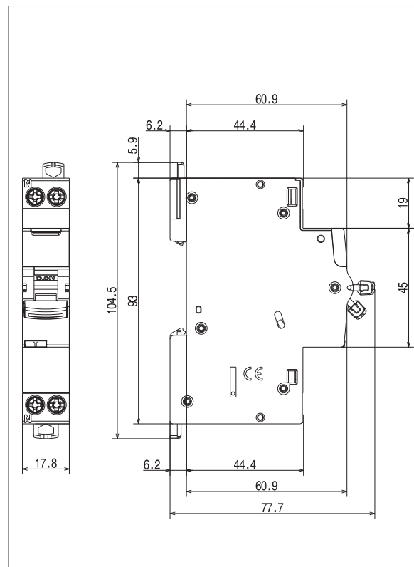
Overall Dimensions
