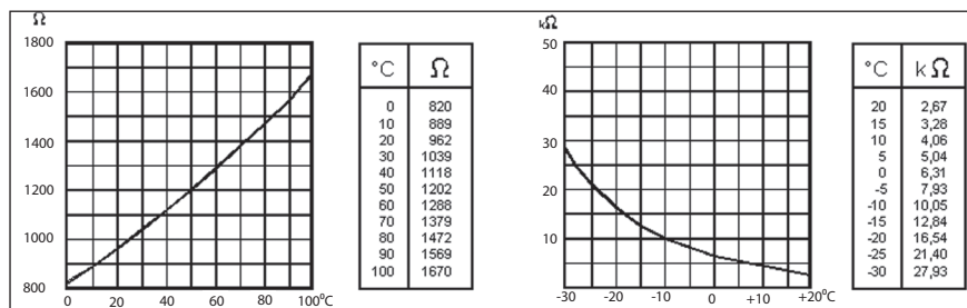
Supply water sensor T1
