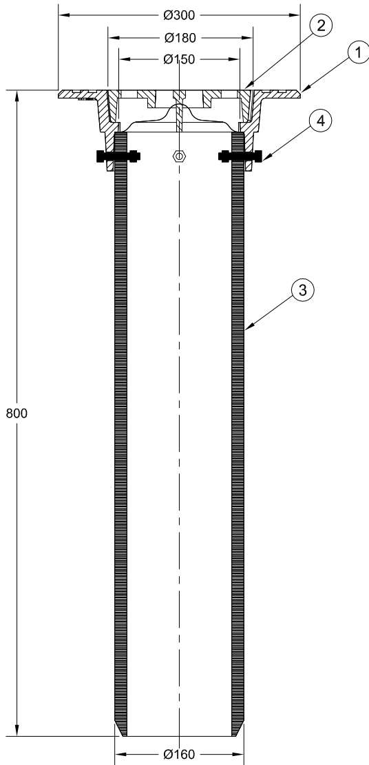
SECTIONAL VIEW X-X
