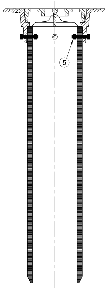
SECTIONAL VIEW Y-Y
