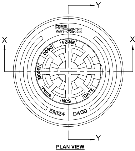
PLAN VIEW
